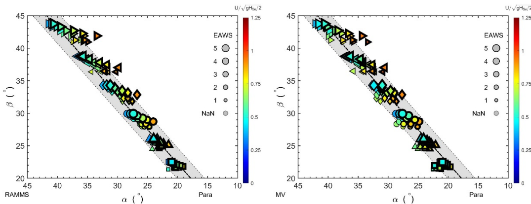
Figure 10 Simulated runout marked by the \alpha -angle and maximum velocity (color coded) on a parabolic track with the mean slope angle, \beta (varying symbol) and snow depth H_S (varying symbol outline) as parameter. Expected runout angle \alpha versus \beta , according to the \alpha - \beta model \alpha_m = 0.96\beta - 1.4^\circ (Lied and Bakkehøi, 1980); gray shaded area \pm\sigma . Simple size gives an impression of the avalanche size according to EAWS volume classification. On the left: RAMMS; on the right MoT-Voellmy.
