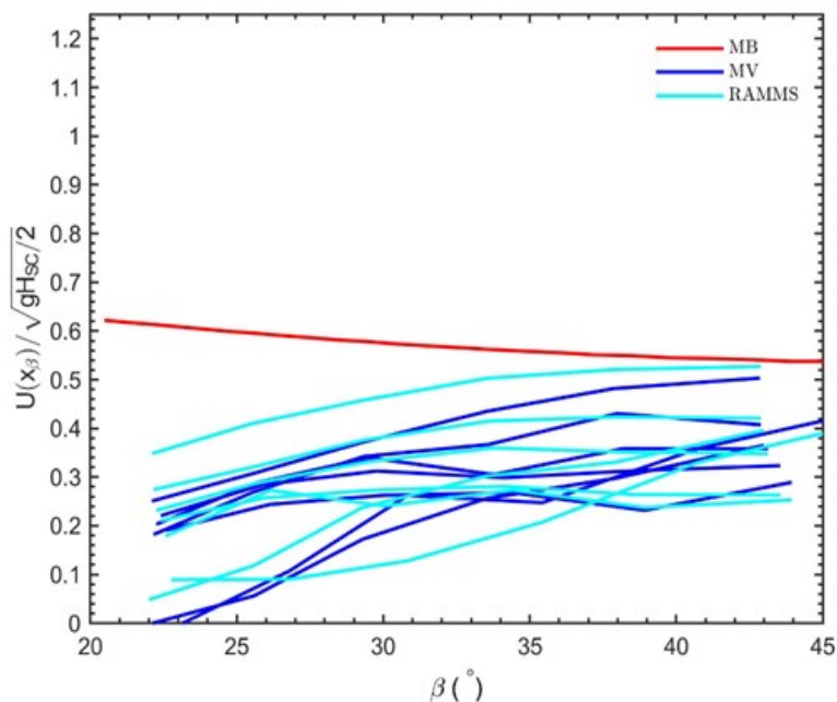
Figure 12 Normalized velocity U = U(x_\beta) / \sqrt{gH_{sc}/2} at the \beta -point for various \beta -angles and different drop-heights.
